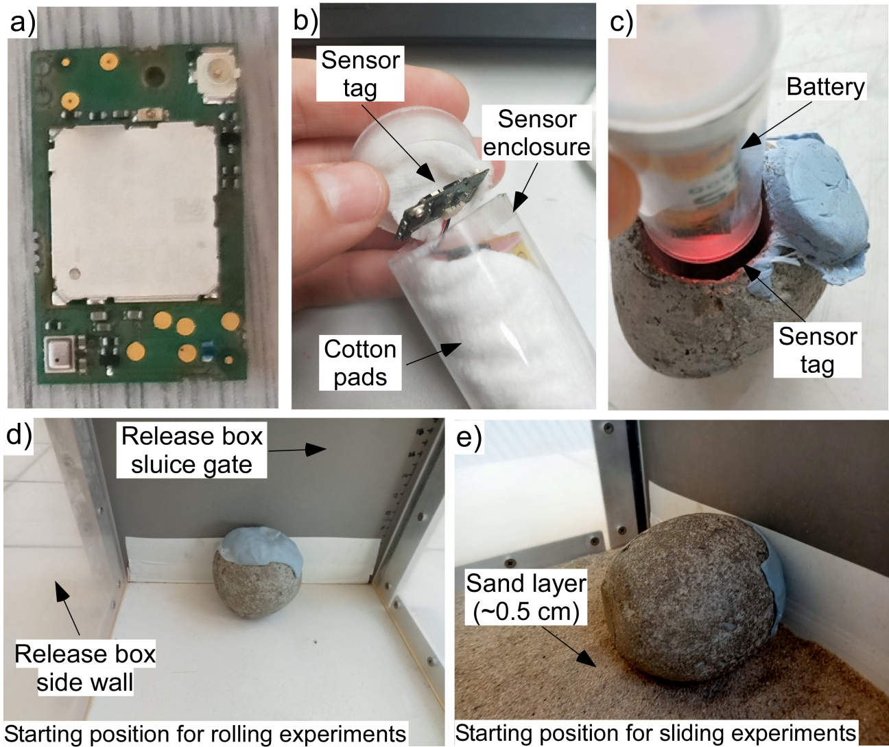
Figure 2 Laboratory experiment pictures. a) Sensor tag. b, c) Sensor installation in the cobble. d, e) The starting position of the cobble within the release box for rolling experiments and sliding experiments while embedded in a thin layer of sand.
