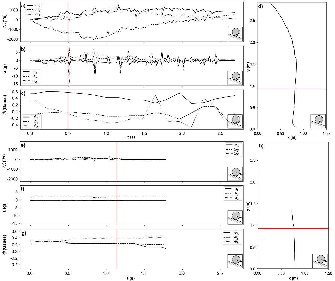
Figure 5 Raw recordings of the three sensor types on a 30° incline for (a, b and c) a rolling experiment (experiment series H1, Table 2) and (e, f and g) a sliding experiment (experiment series H2, Table 2). a, e) gyroscopes data. b, f) accelerometers data. c, g) magnetometers data after upsampling. The solid line refers to the x axis, the dashed line to the y axis and the dotted line to the z axis. Trajectories extracted from camera videos for (d) rolling tests and (h) sliding tests carried out on a 30° incline. The solid red line shows the time when the cobble passes over the slope break.
