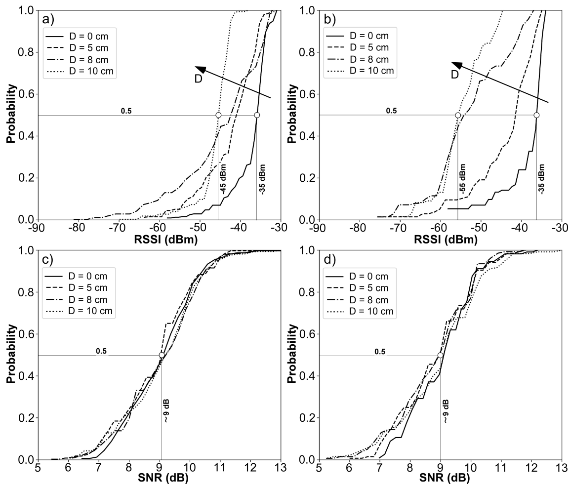
Figure 4 Cumulative probability distribution of (a and b) Received Signal Strength Indicator (RSSI) and (c and d) Signal Noise Ratio (SNR) when the signal is transmitted through different sand layer depths, namely 0 cm, 5 cm, 8 cm, and 10 cm (experiment series A-E, Table 2). RSSI and SNR are measurements of the signal power received in the gateway and the ratio of the signal power and the noise power, respectively. a, c) Accelerometer and gyroscope packets. b, d) Magnetometer packets.
