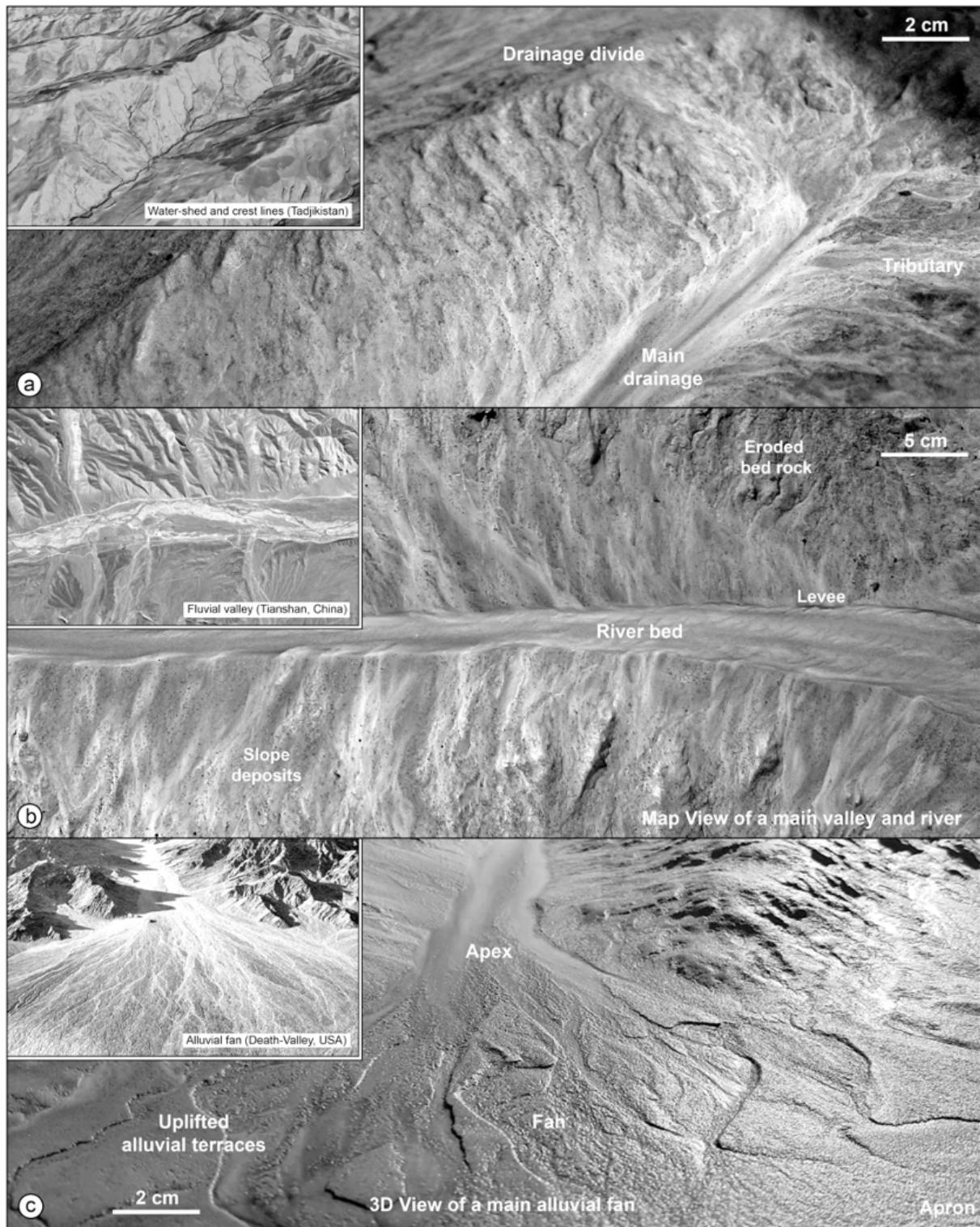
Figure 14 Selection of experimental morphologies obtained with the MAT-V standard composition. a) 3D view of the upper portion of a main watershed showing crest lines and drainage divide morphologies. b) Map view of a main channel situated in the lower portion of a large catchment. Note the diversity of sedimentary bodies distributed along the channel. c) 3D view of a large alluvial fan developing at the front of the relief area, and spreading over the foreland basin. Several alluvial surfaces of different abandonment ages can be observed.
