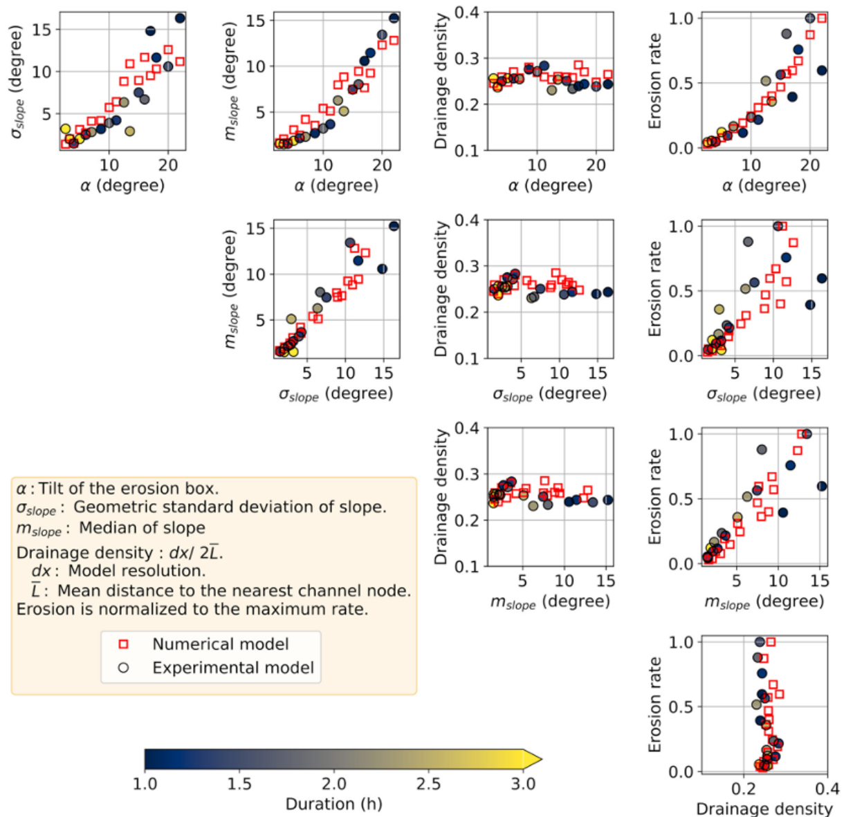
Figure 12 Relationship between geomorphological features characterizing the best agreement between experimental (circles) and numerical (red squares) models. All proxies are dimensionless. The tilt angle of the erosion box is \alpha . The geometric standard deviation and median of the slope change distribution observed at the surface are \sigma_{slope} and m_{slope} , respectively. Drainage density is estimated at each node based on the mean distance to the nearest channel node (Tucker et al., 2001). Erosion rates are normalized to the maximum observed rate. The color scale indicates the duration of each experiment.
