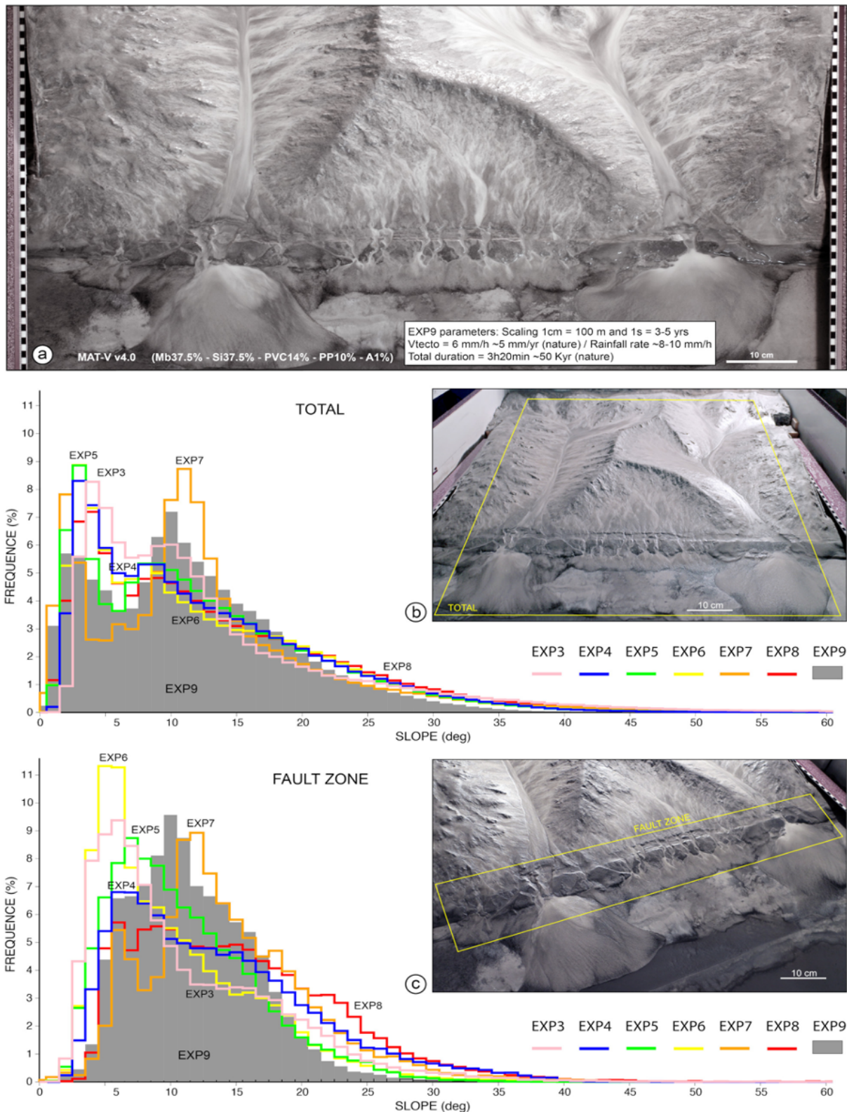
Figure 4 Example of morphometric measurements used to quantitatively determine the optimal MAT-V composition. a) General 2D view of the final stage of EXP 9. MAT-V composition and experiment parameters are indicated. b) and c) Comparison of model surface slope distributions for EXP 3, 4, 5, 6, 7, 8, and 9 for the entire model (Fig. 4b) and within the fault zone only (Figs. 4c).
