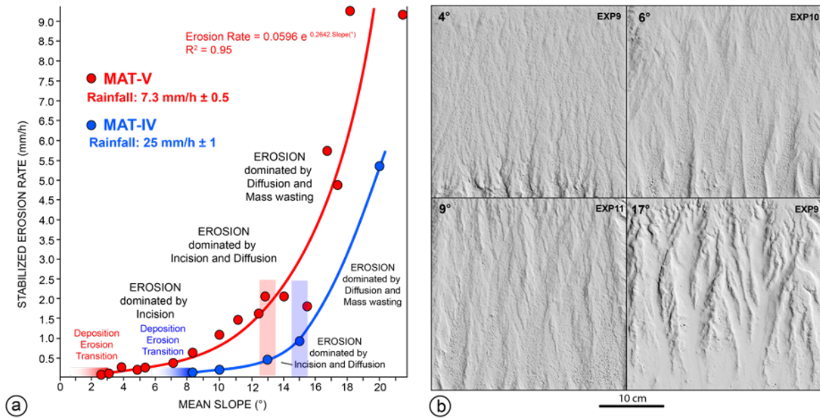
Figure 10 Comparison between MAT-IV and MAT-V erodibility as a function of mean slope. a) Stabilized erosion rates versus mean topographic slope. b) Examples of erosion box morphologies for different initial slopes (standard MAT-V composition) during steady-state erosion phases.
