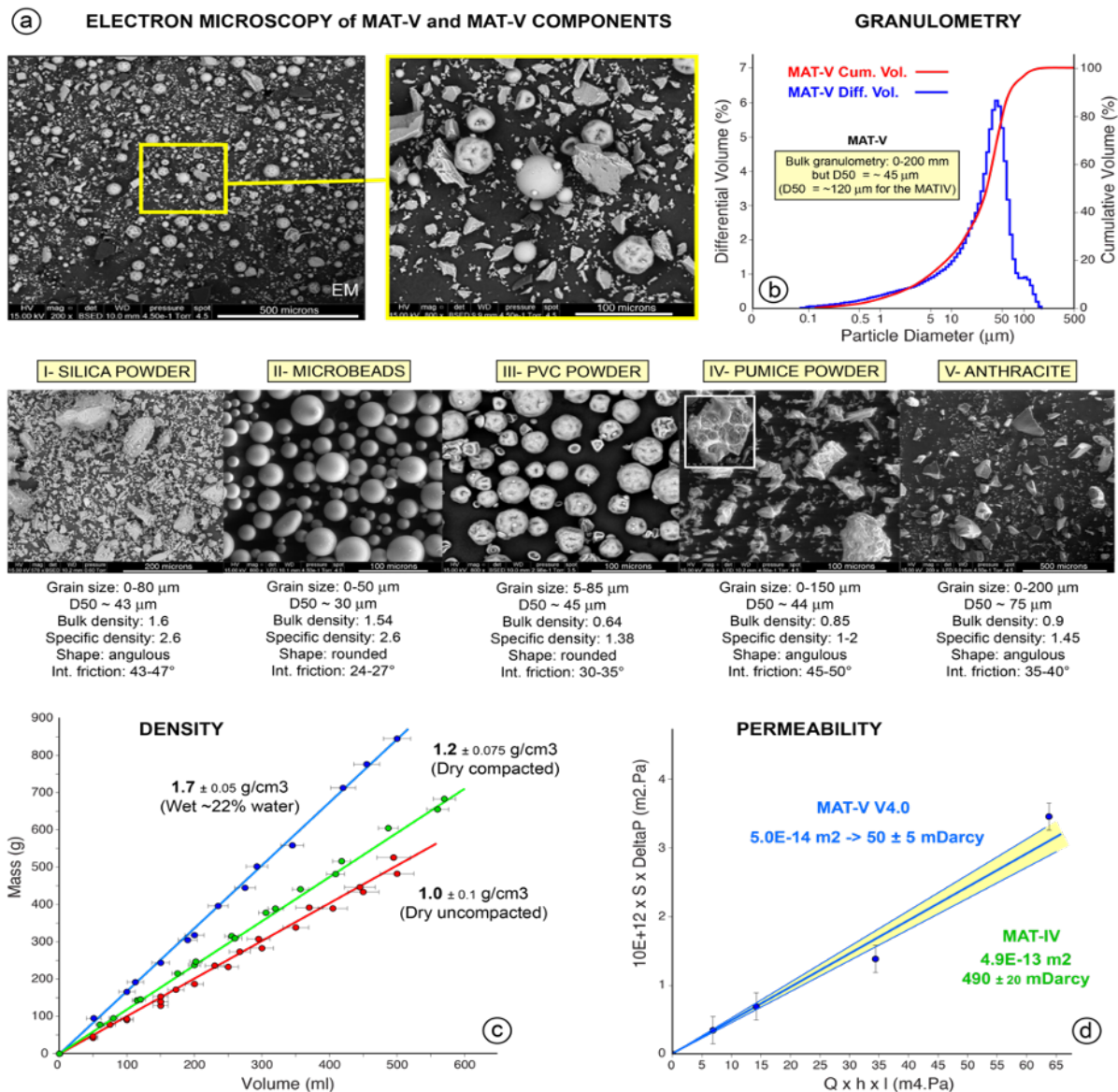
Figure 6 Physical properties of the MAT-V analog material: a) Particle shapes, as observed at microscopic scale (SEM). b) MAT-V granulometry. c) Bulk densities of MAT-V under wet (at 22% by mass of water) and dry (compacted and uncompacted) conditions. d) MAT-V permeability measured using Darcy's pipe permeameter.
