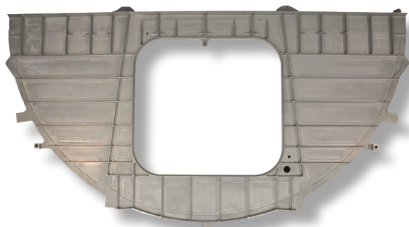
Alcoa bulkhead prototype from Lunar Module, c. 1969. Before Neil Armstrong descended the ladder to reach the lunar surface, he exited Lunar Module Eagle through an aluminum hatch door.
